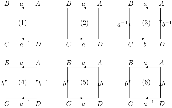
Figure 1.6. Construction of surfaces from I \times I
