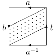
Figure 1.7. Möbius band in the Klein bottle
